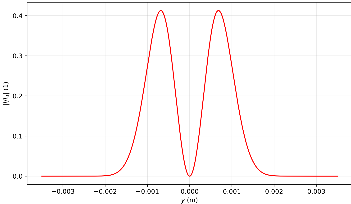
Intensity profile I(x=0, y, z=1.911)/I_0 , \text{Pin}=0.5\text{Pcr} , artificial time
